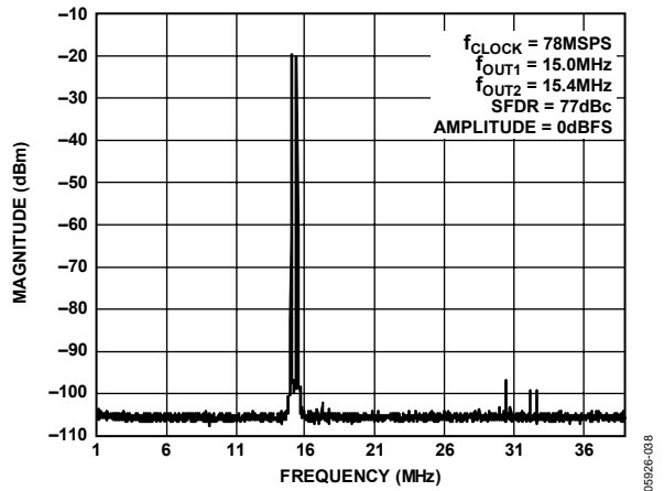
Figure 42. Dual-Tone SFDR
