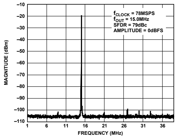
Figure 24. Single-Tone SFDR
