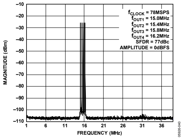
Figure 43. Four-Tone SFDR
