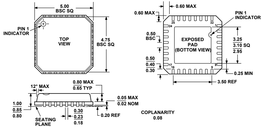
Figure 103. 32-Lead Lead Frame Chip Scale Package [LFCSP_VQ] 5 mm × 5 mm, Very Thin Quad (CP-32-2) Dimensions shown in millimeters
